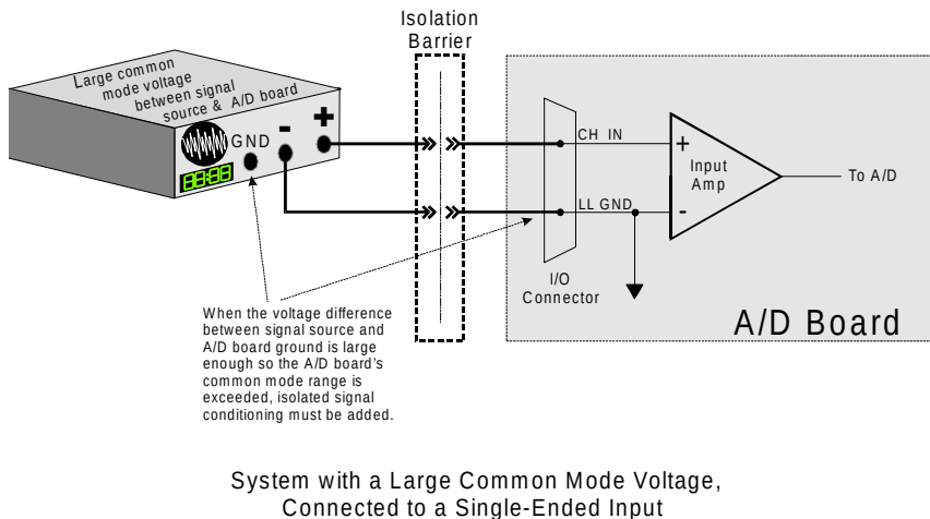
Figure 5-8. Common Mode Voltage Greater Than \pm 10V , Single-Ended Input w/Isolation Barrier
