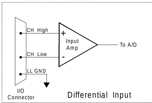
Figure 5-2. Differential Input - Common Mode Voltage Rejection
