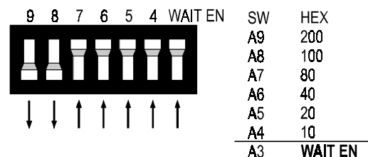
Figure 3-1. Base Address Switches
