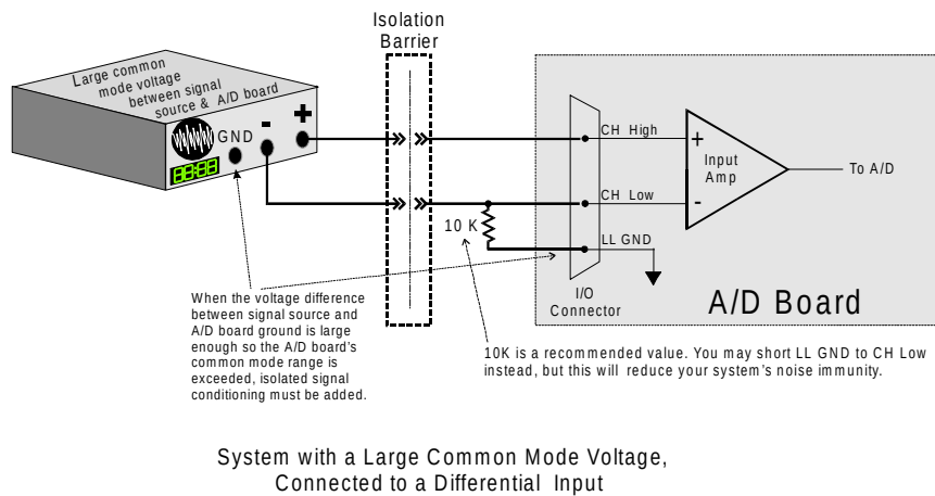
Figure 5-7. Common Mode Voltage Greater Than \pm 10V , Differential Input
