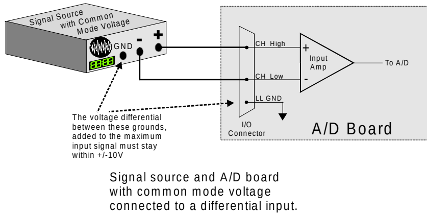
Figure 5-6. Differential Input, Maximum Common Mode Voltage Requirement
