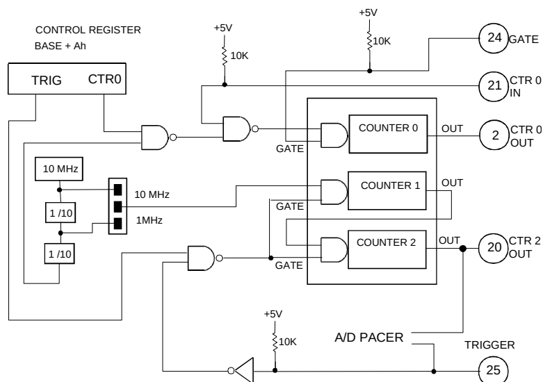
Figure 6-2. Pacer and Counter Block Diagram
