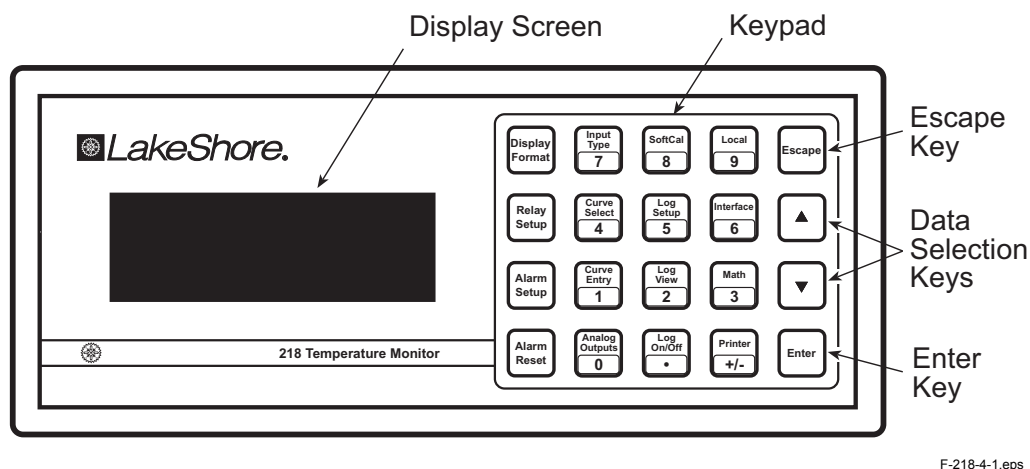
Figure 4-1. Model 218 Front Panel
