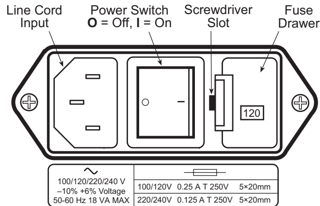
Figure 7-1. Power Fuse Access
