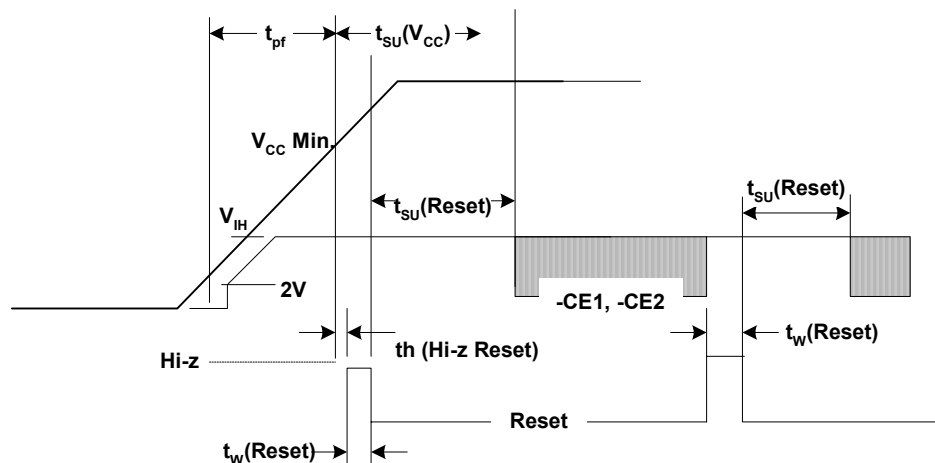
Figure 3-1. Power-Up Timing for Systems Supporting RESET
