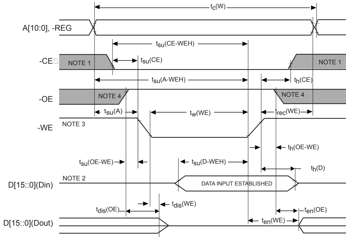
Figure 3-4. Common and Attribute Memory Read Timing Diagram
