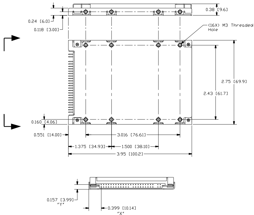
Figure 2-4. FlashDrive Dimensions
